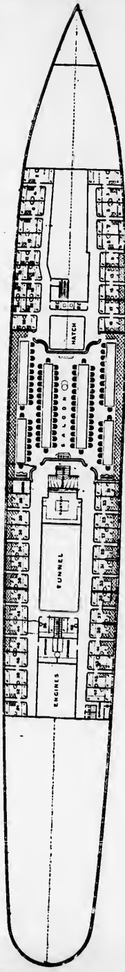
DECK PLAN OF SS. OCEANIC. (The first Atlantic Steamer with a midship saloon.)
